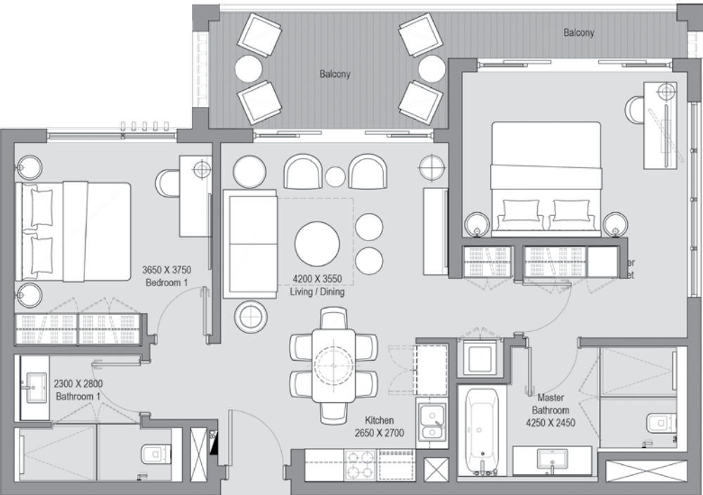
THIRD LEVEL
