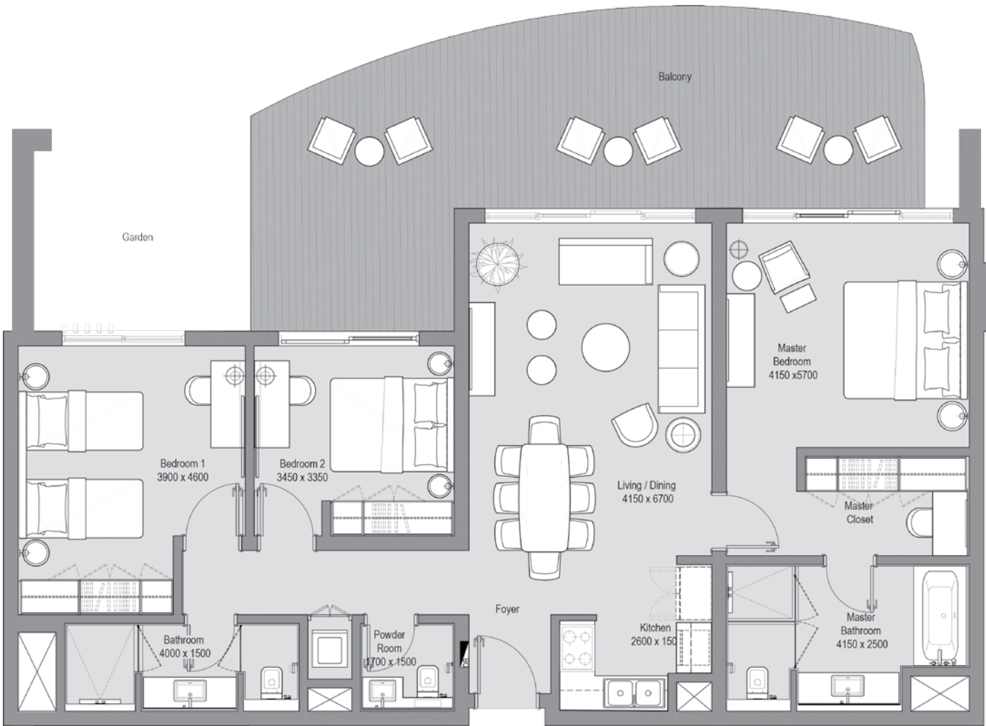
GARDEN LEVEL
