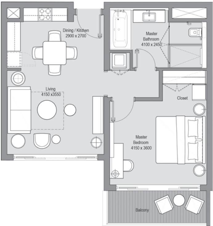
SECOND LEVEL
