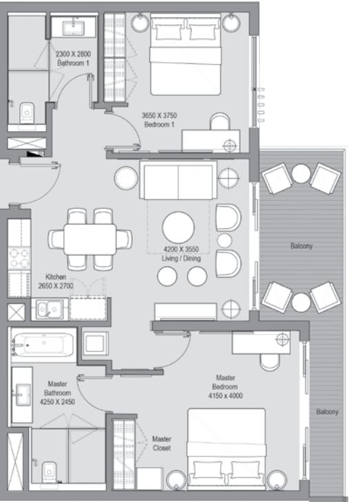
SECOND LEVEL
