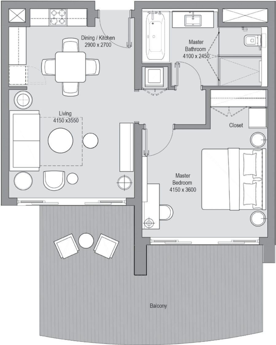
GARDEN LEVEL
