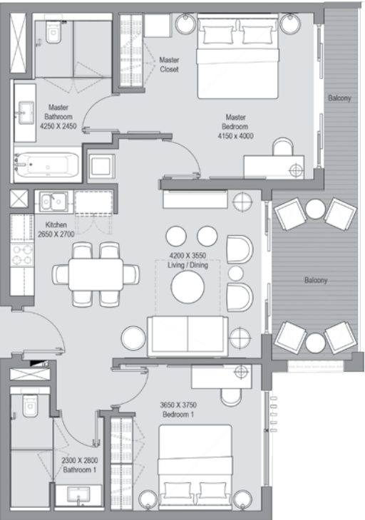
THIRD LEVEL
