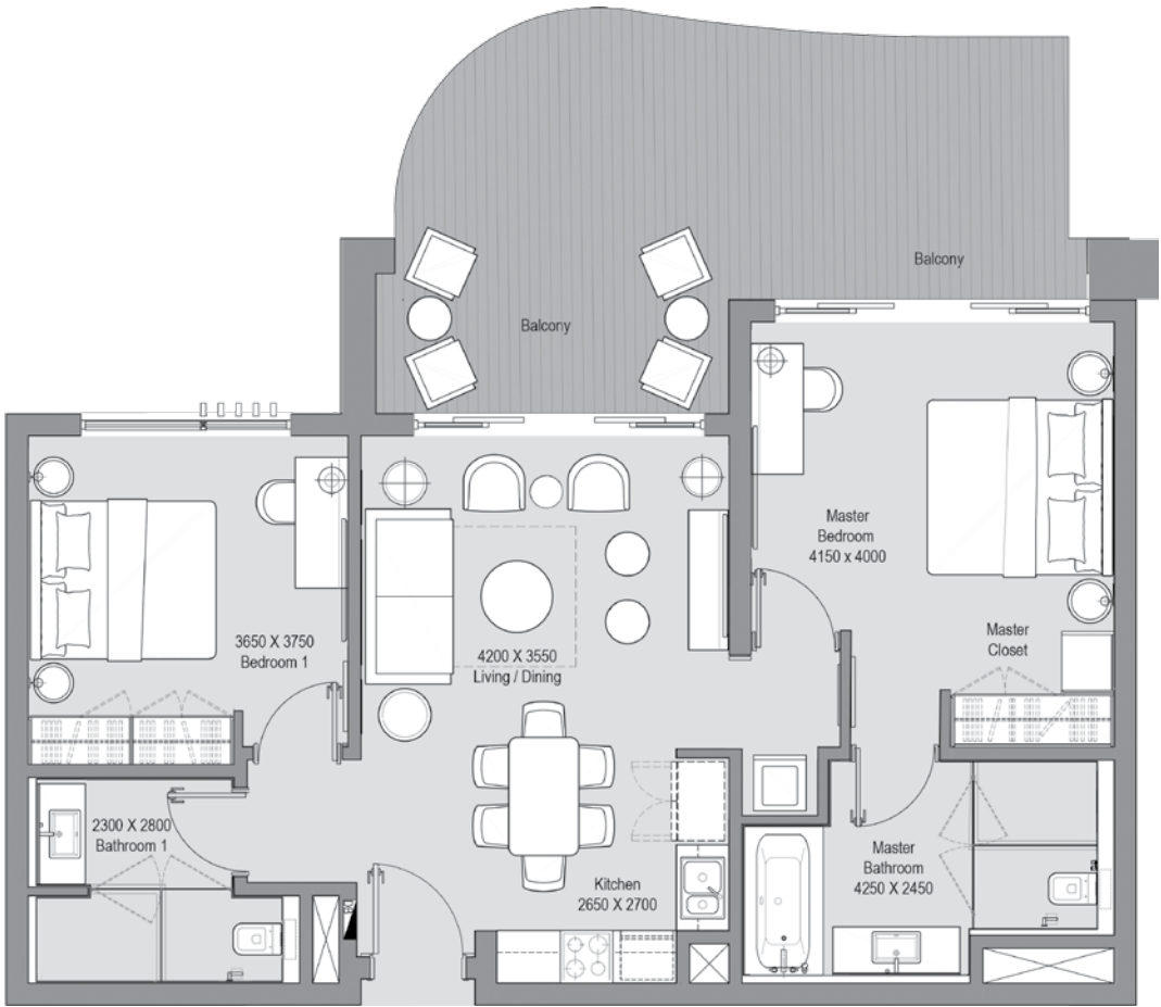
GARDEN LEVEL
