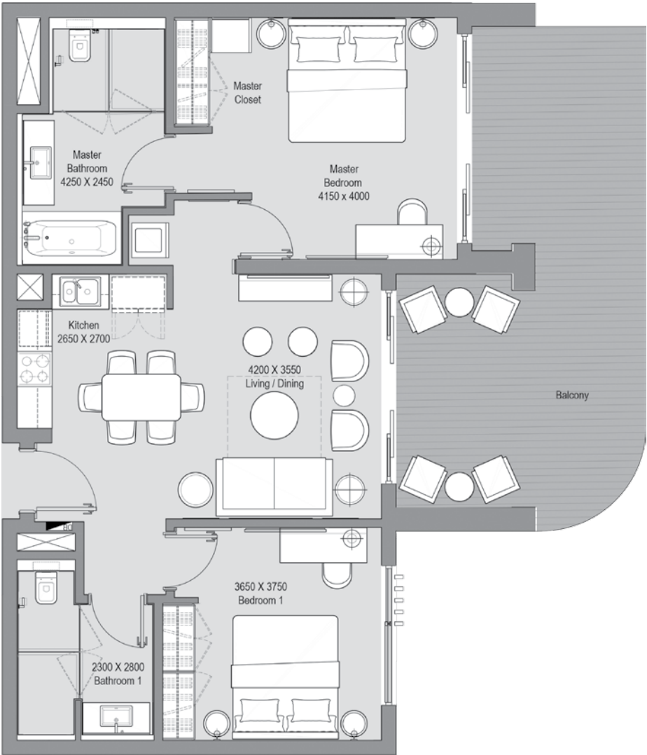
GARDEN LEVEL
