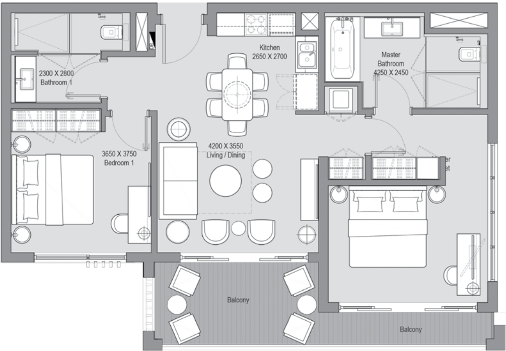
SECOND LEVEL
