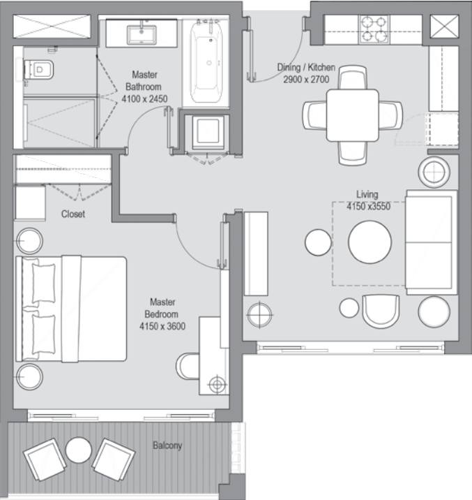
THIRD LEVEL
