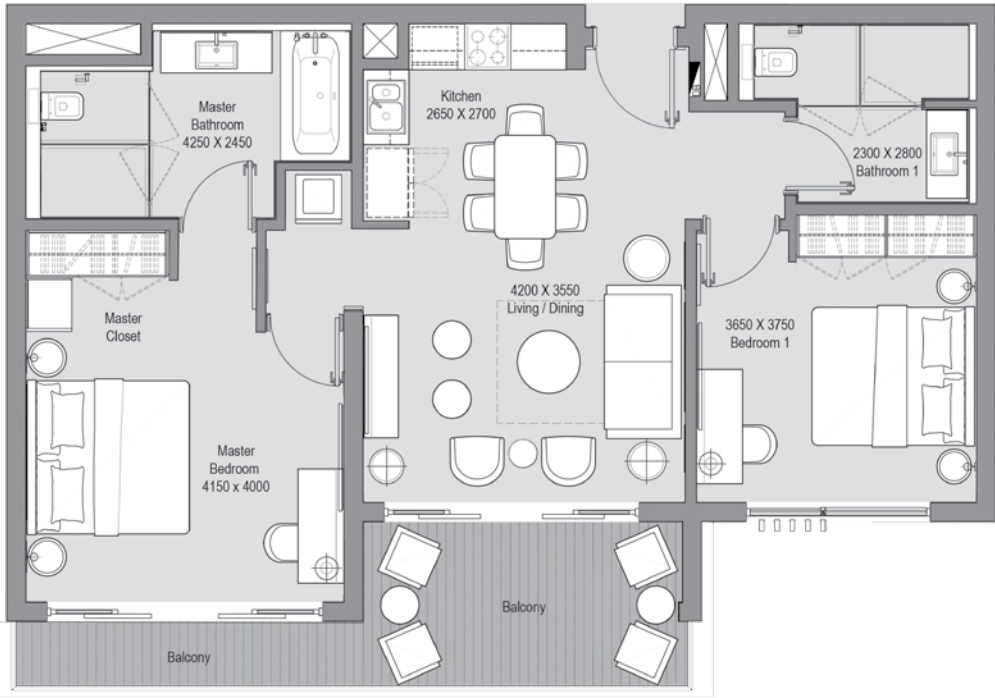
THIRD LEVEL
