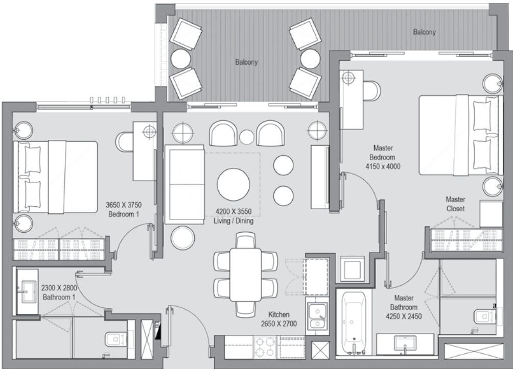
FIRST LEVEL
