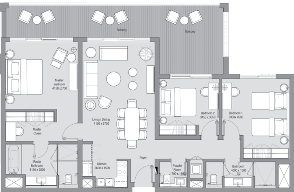
THIRD LEVEL
